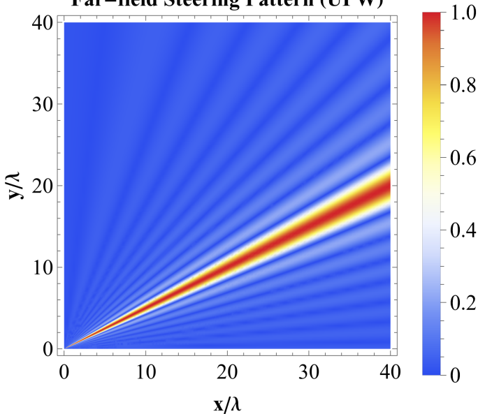
Far-field Steering Pattern (UPW)
